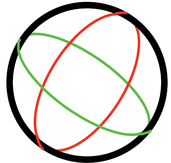
After 20 epochs
