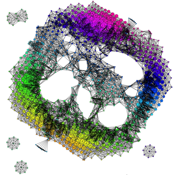
After 20 epochs
